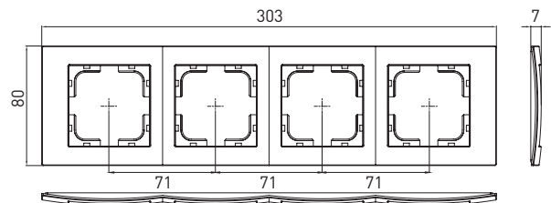
4 Gang Frame
